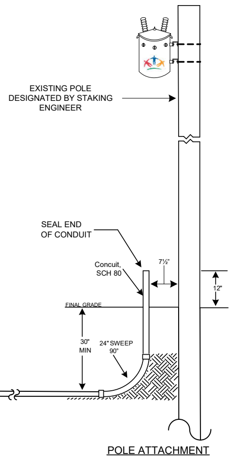
POLE ATTACHMENT
