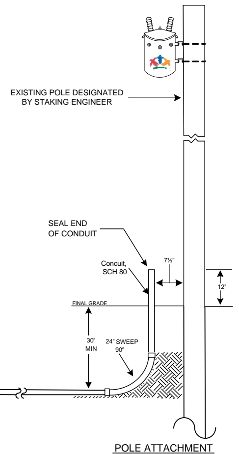
POLE ATTACHMENT
